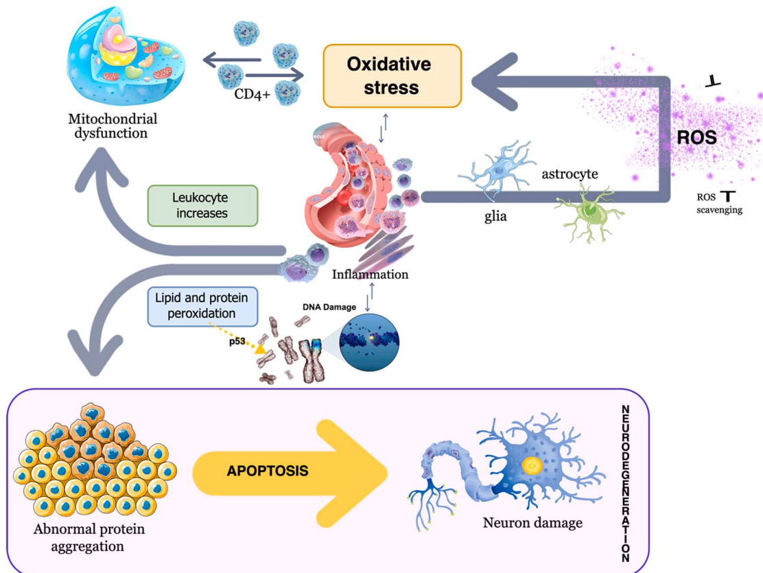
Fig. 3. Neurodegeneration pathway.
