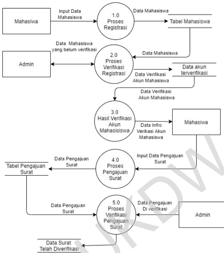
Gambar 3.3 DFD Level 1
